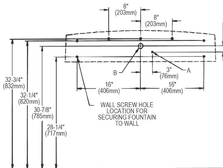
WALL LAYOUT
