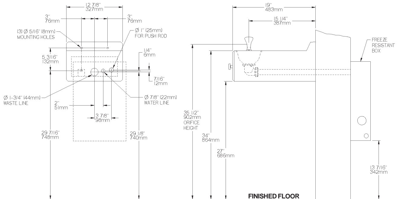
4593FR ROUGH-IN
