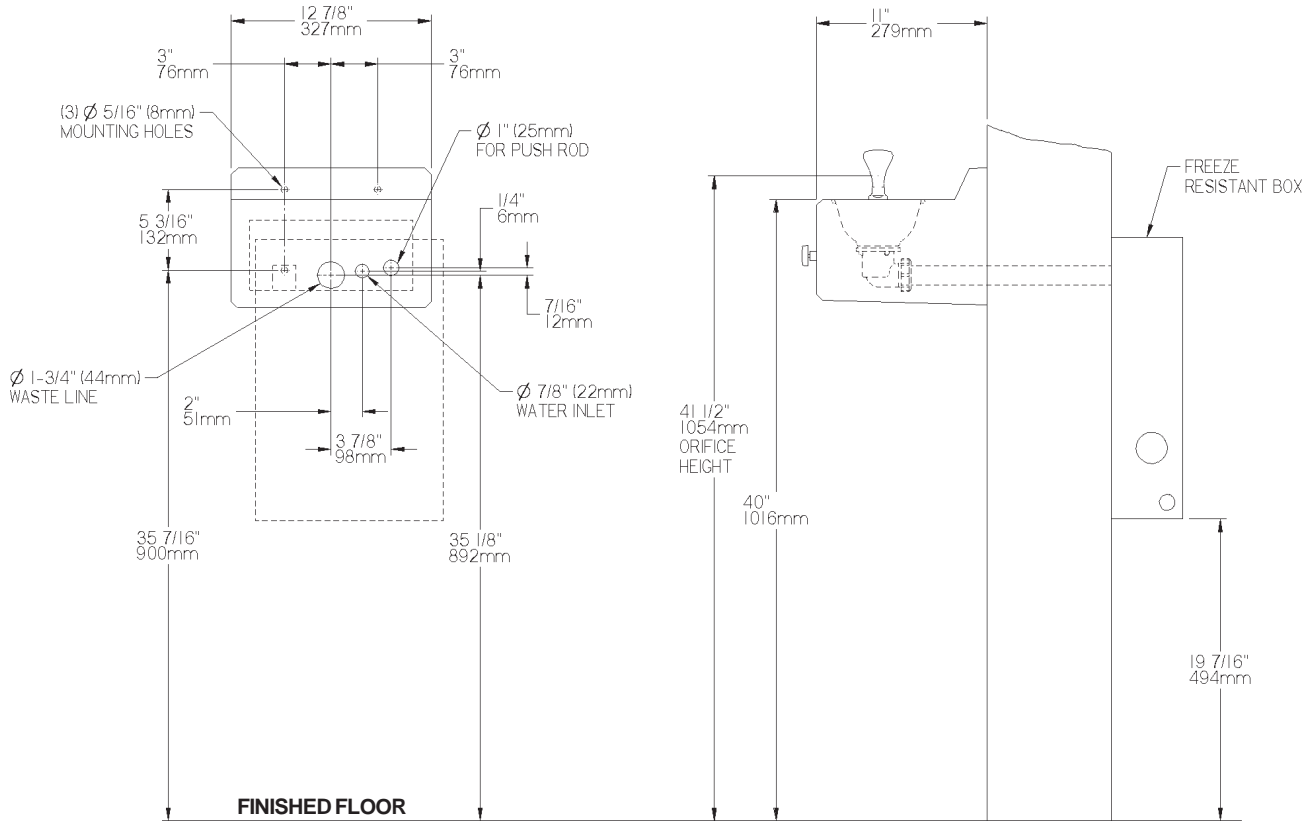
4592FR ROUGH-IN
