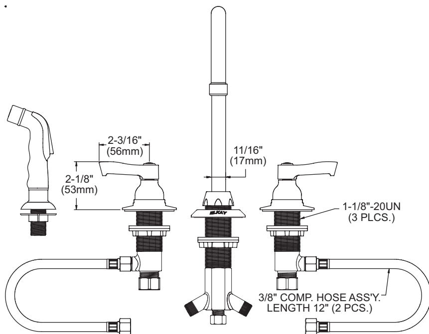
Model LK801GN08T2 FRONT VIEW
