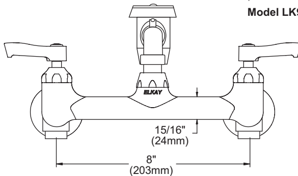
Model LK940BP03L2S FRONT VIEW
