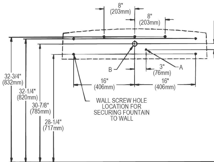
WALL LAYOUT
